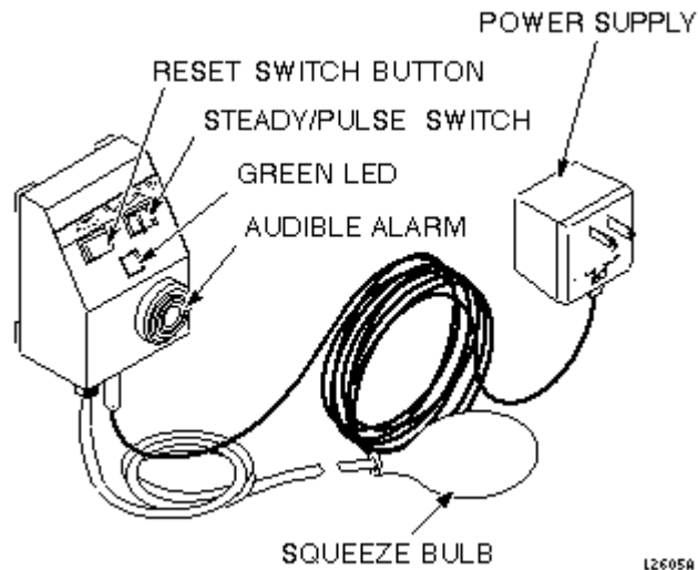
CONTROL AND INDICATOR LOCATIONS ILLUSTRATION 1-1
